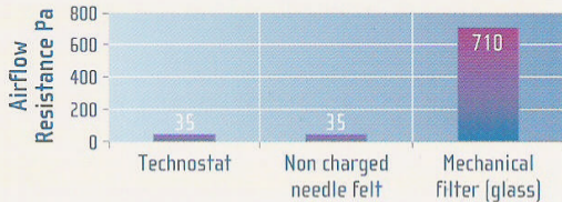
Airflow Resistance
