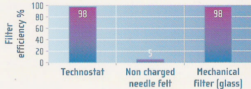
Filter Efficiency
